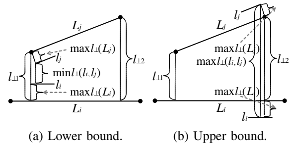
Fig. 15. Derivation of the bounds for d_{\perp} .
